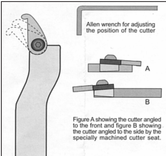
The Mushroom Tool is fitted with the Mushroom cutter and comes with an Allen key for cutter adjustment.
