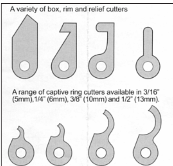
There are many additional cutters available including a range of captive ring cutters.
