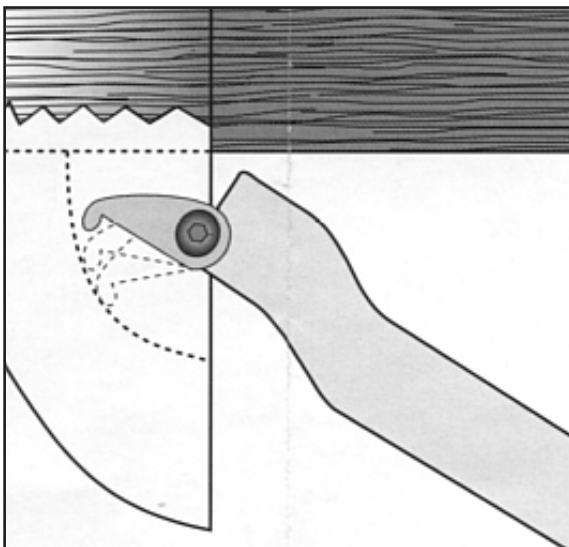
Continue undercutting using a sweeping action to produce a smooth underside.
